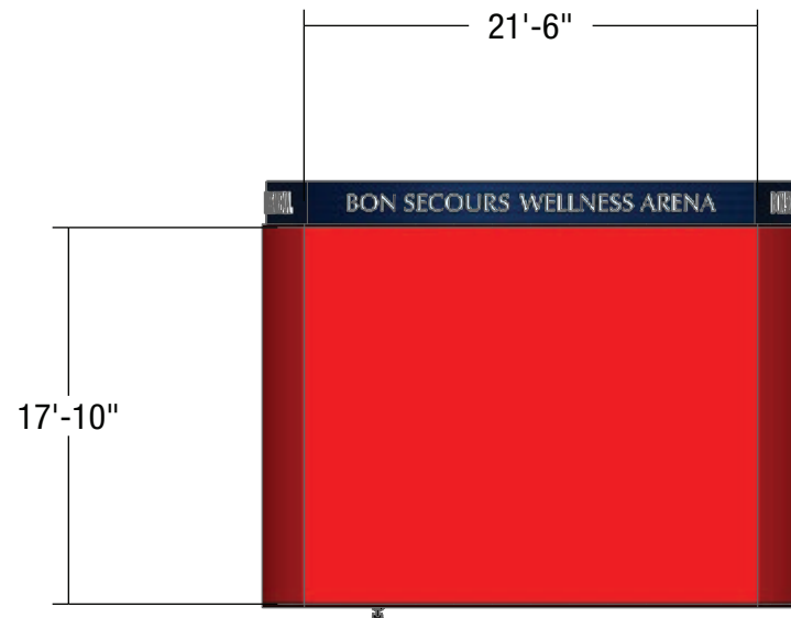
LAYOUT ENDZONE 1" = 10' (1:120)
