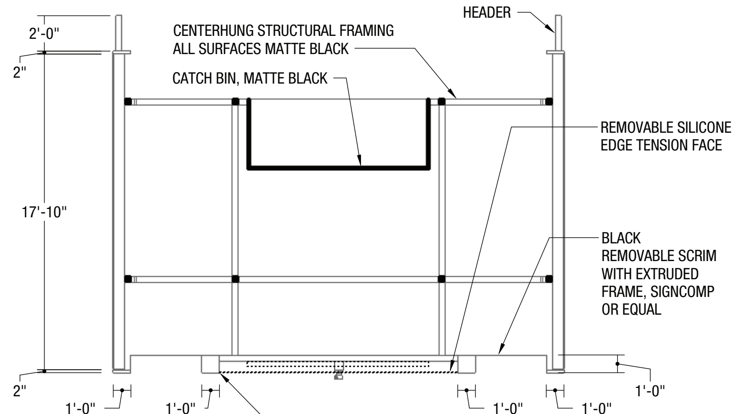
SECTION 3/16" = 1'-0" (1:64)
