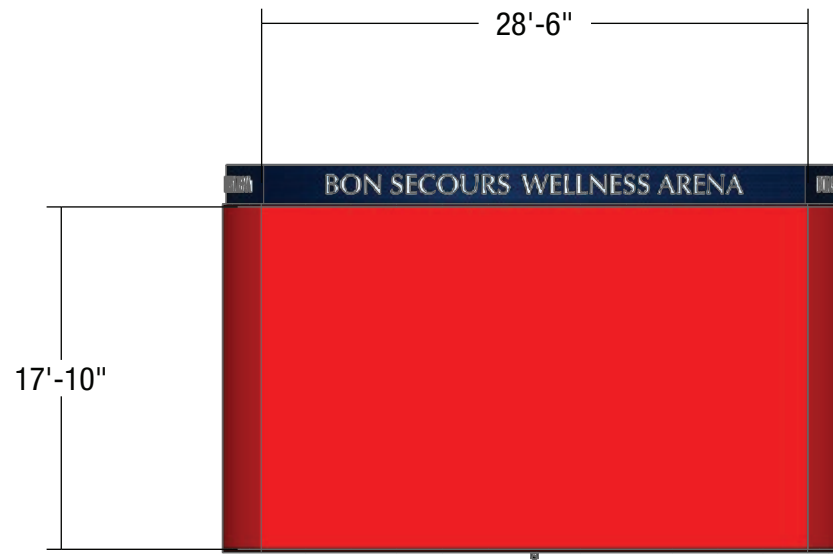
○ LAYOUT SIDELINE 1" = 10' (1:120)
